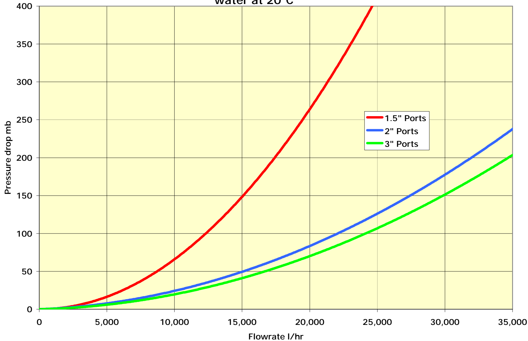
Flowrate v. Pressure drop - Axiom Pure-Screen 100 - 250 micron filter with water at 20°C
